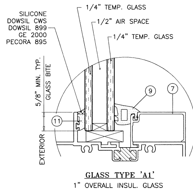
GLAZING OPTIONS INTERIOR GLAZED
