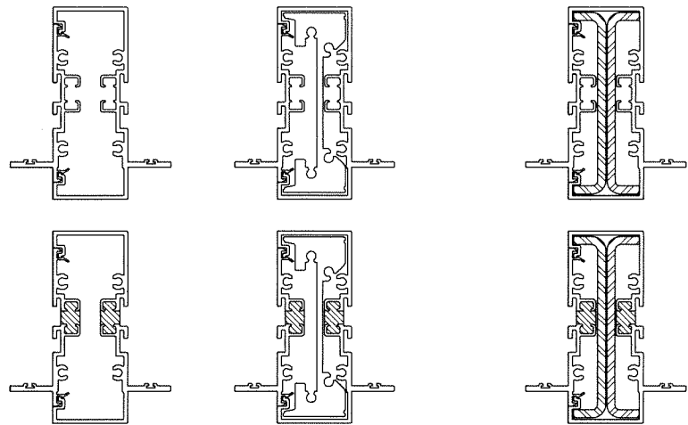
MULLION 'M1'
