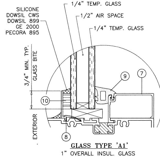
GLAZING OPTIONS EXTERIOR GLAZED
