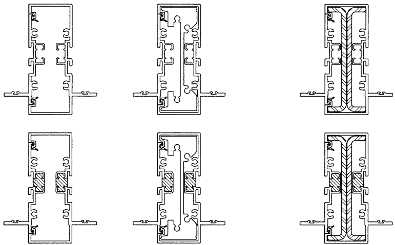
MULLION 'M1'
